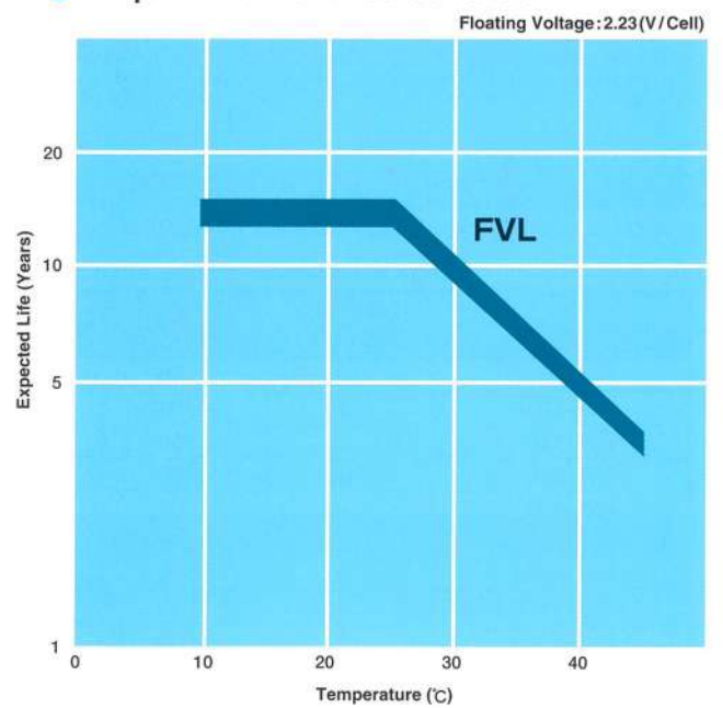
● Temperature-Life Characteristics
